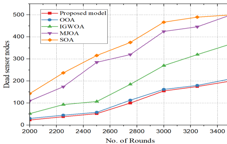
Fig 8. Dead sensor nodes comparison between existing and proposed model.
