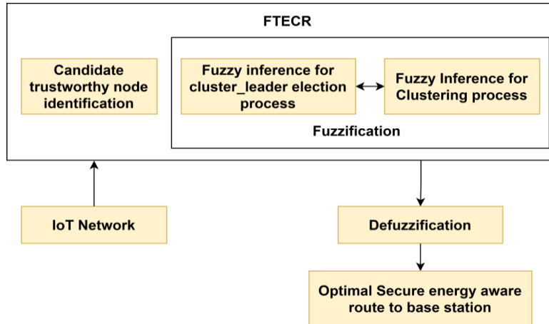
Fig 2. Fuzzy Inference System.
