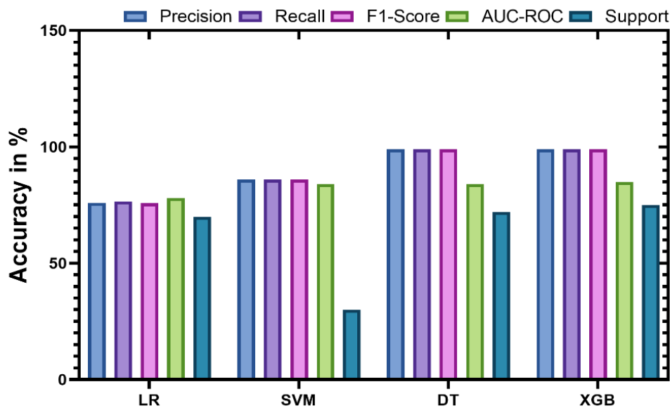
Fig 5. Comparative Analysis of Various ML In the Prediction of Diabetics.
