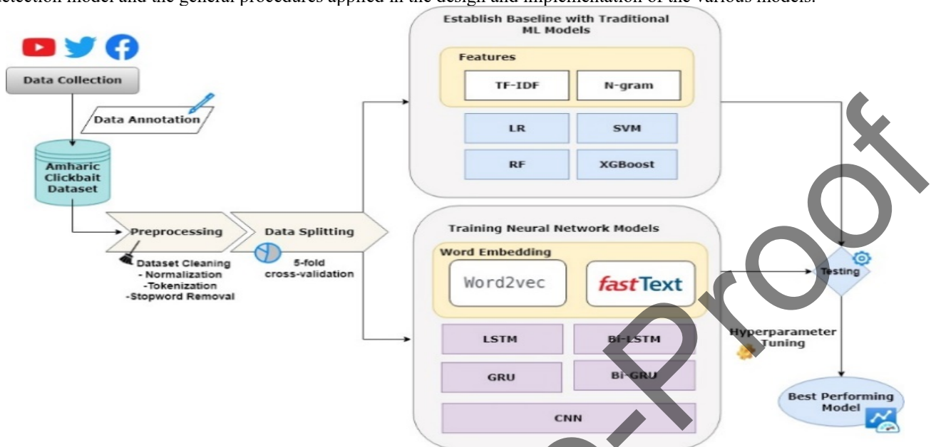
Figure 3. Architecture of the Proposed Clickbait Detection Model
