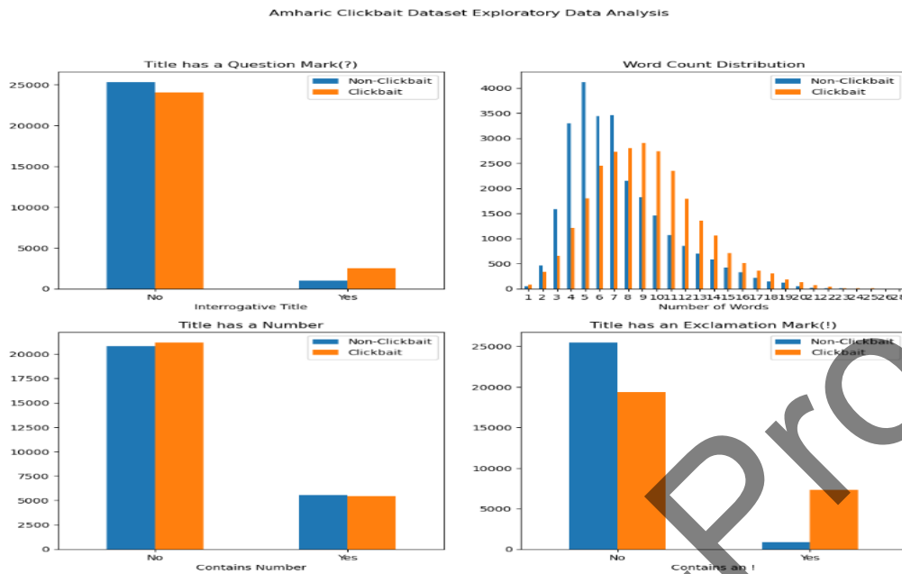
Figure 2. Exploratory Data Analysis Results of the Amharic Clickbait Dataset
