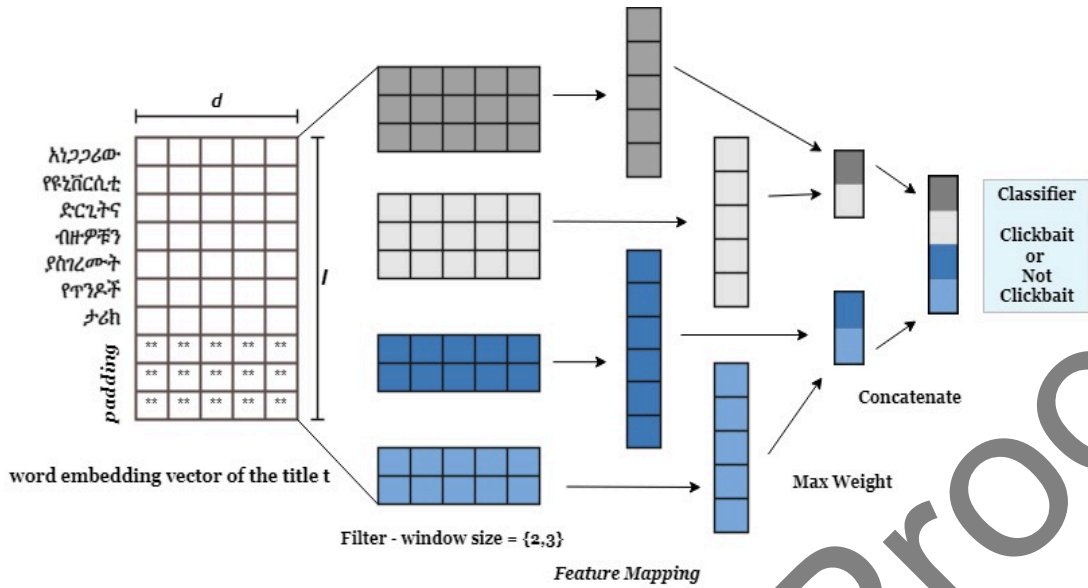
Figure 4. CNN Architecture for Feature Extraction of Amharic Clickbait Detection
