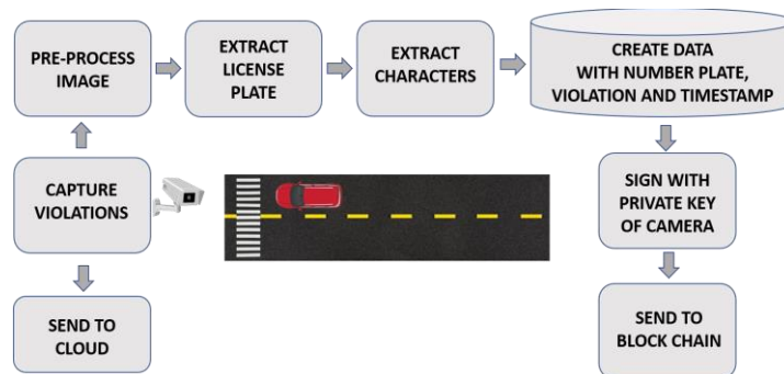
Fig 2. functions of IoT camera
