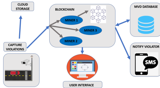
Fig 3. Architecture diagram
