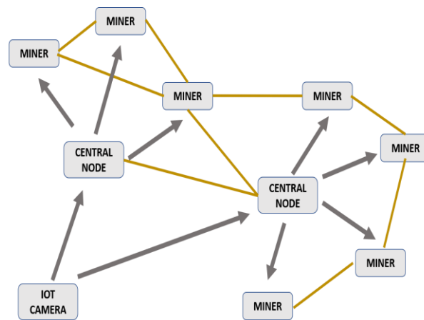
Fig 1. Blockchain Network
