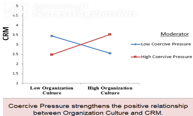
Fig 4. Interaction effect of coercive pressure on organizational culture and construction risk management
