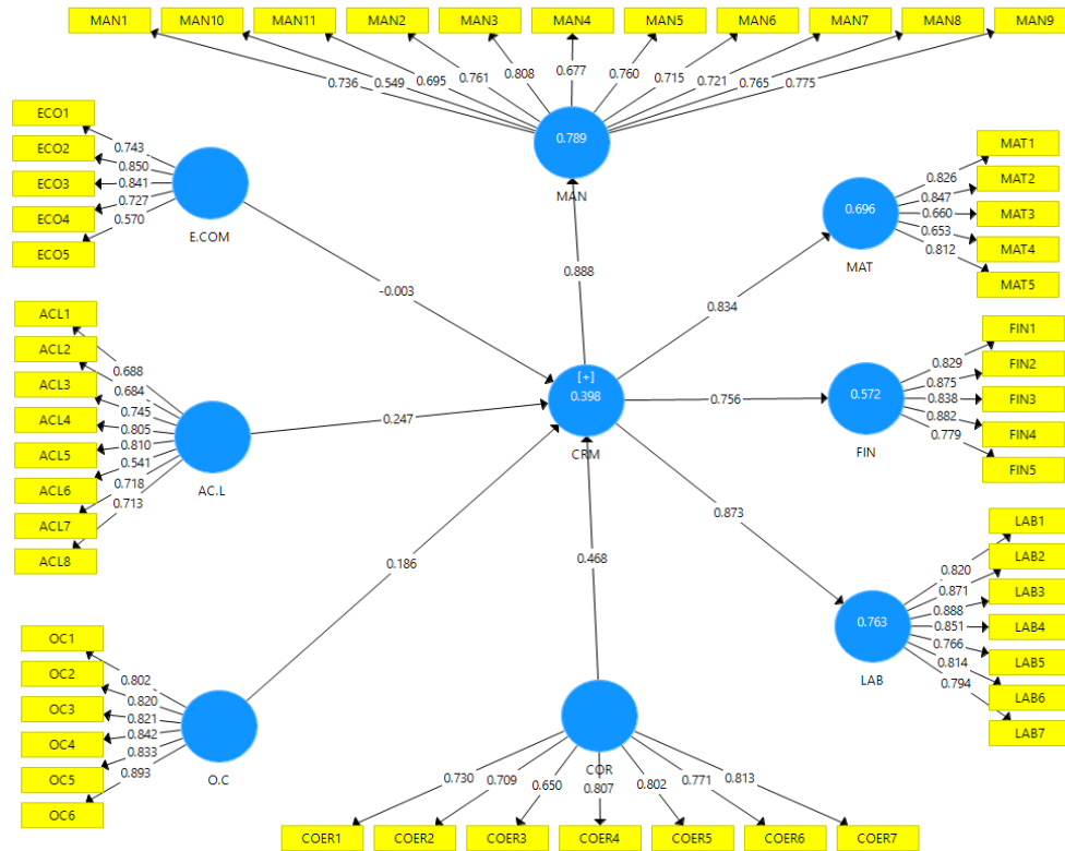
Fig 2. The evaluation of structural model through PLS
