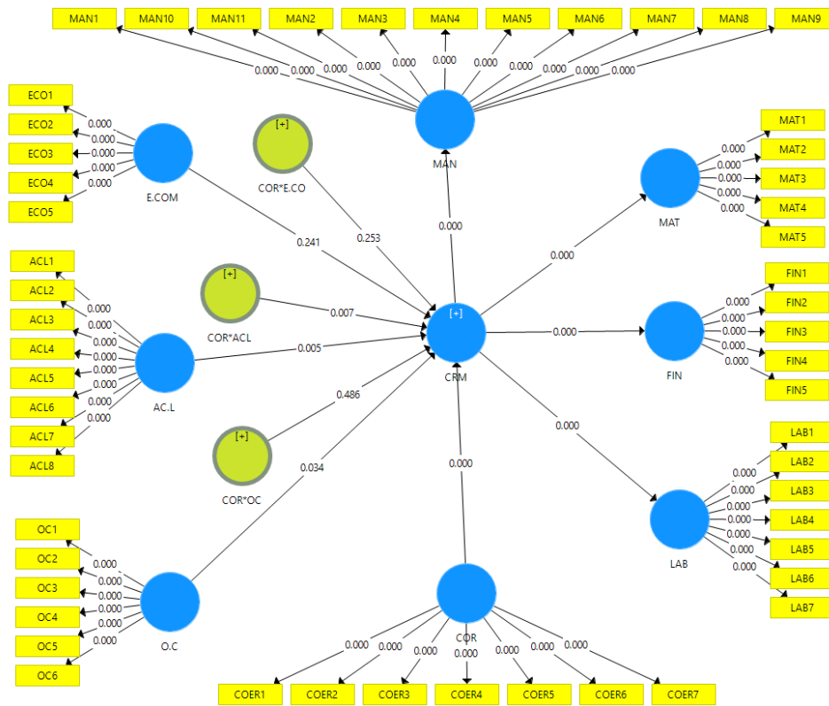
Fig 3. The evaluation of structural model through PLS bootstrapping
